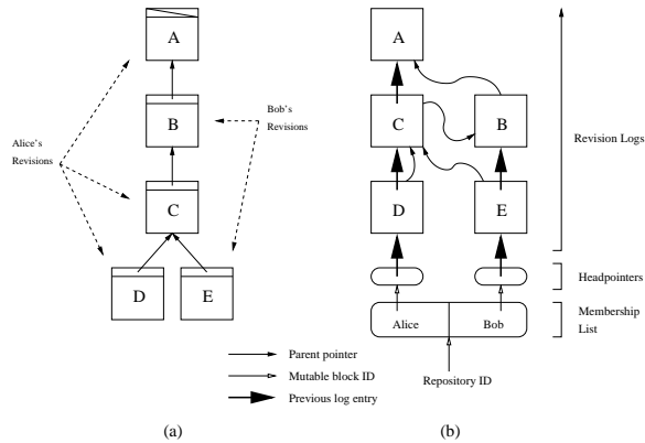
Figure 9: DHT storage structures. (a) shows an example revtree. (b) shows the same revtree, as stored in the DHT. Rounded rectangles are mutable blocks and square rectangles are immutable blocks.
