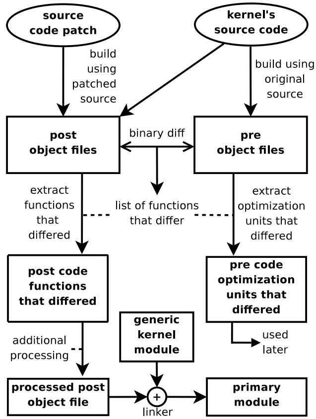
Figure 1: Generating replacement code based on a patch (Part I of generating a Ksplice hot update)
